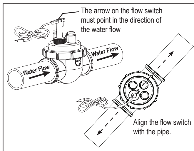
Figure 3. Replacing the Flow Switch
