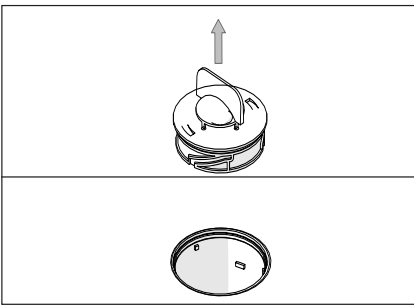
Figure 2. Remove Existing Lens
