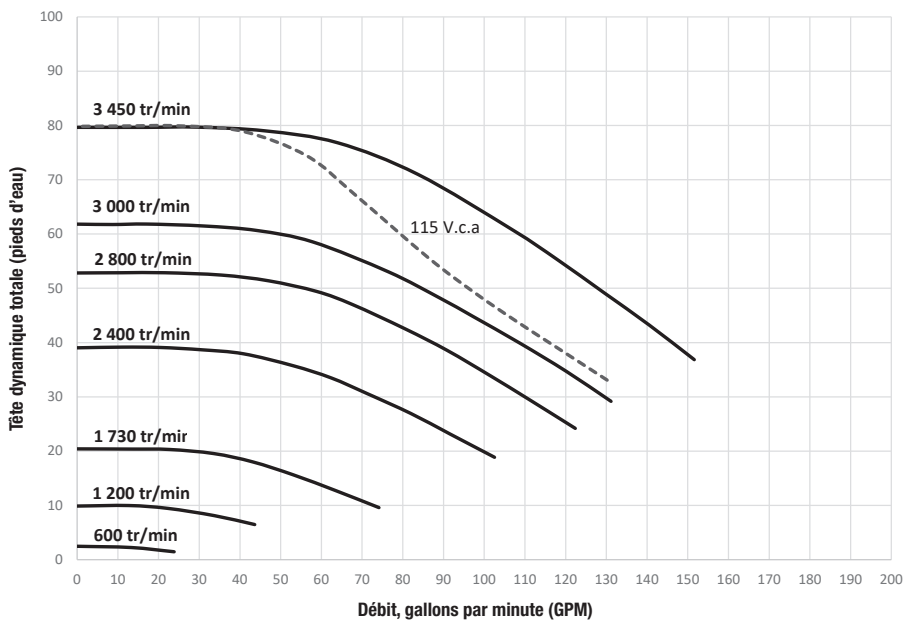
Courbes de performance VSSHP220DV2A(S)
