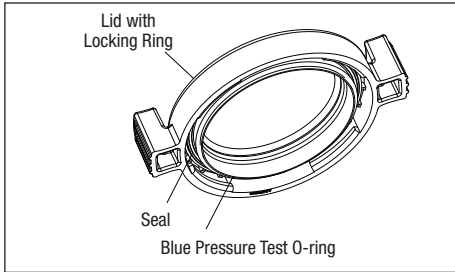
Figure 14. Blue Pressure Test O-ring
