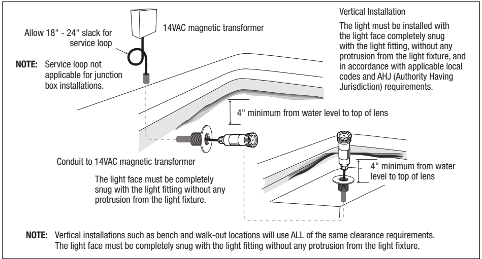
Figure 3. Standard installation with 1.5" pool wall fitting
