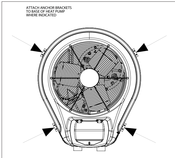
Figure 1. Anchor Clamp Positions
