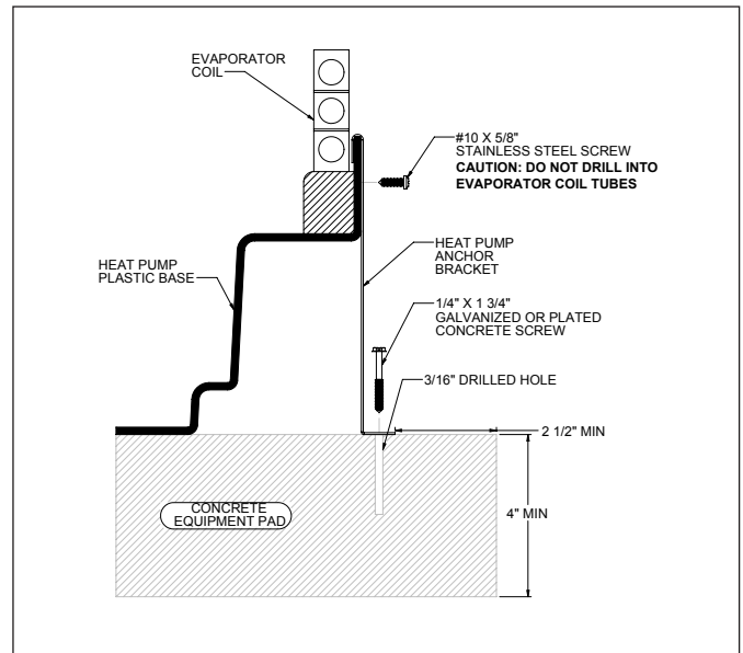
Figure 2. Anchor Clamp Installation
